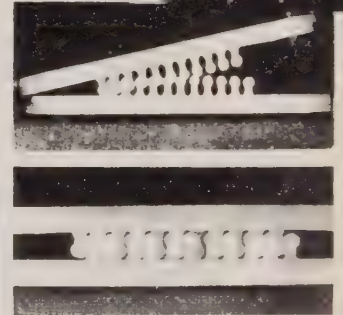
Smooth surfaces of nylon or acetal snap together without need for precise alignment. They hold firmly until pulled apart by a specified force.
